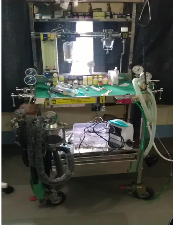
BOYLES APPARATUS
